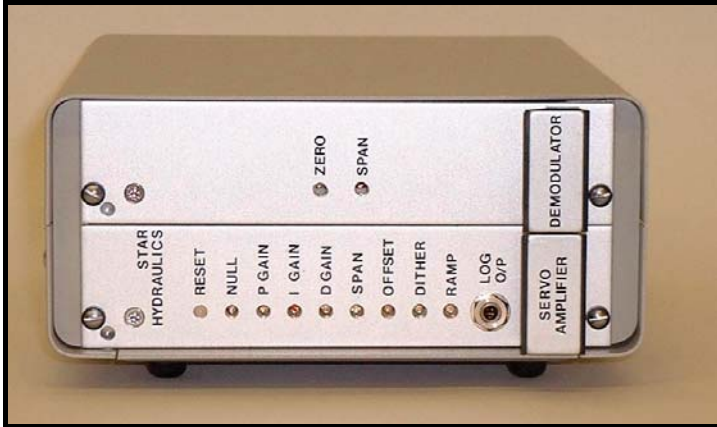
STE3010 Front Panel
