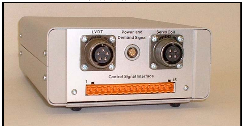
STE3010 Rear Panel
