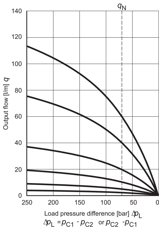
Output flow versus load pressure difference
